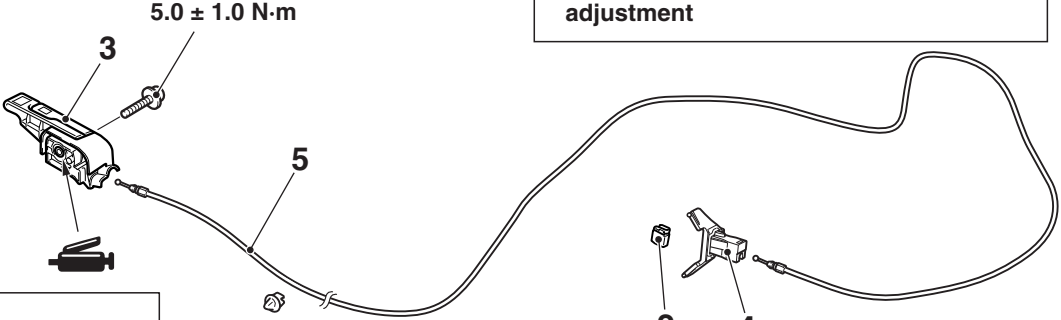
Fuel filler lid height and clearance adjustment
