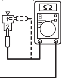
Resistor harness side connector (front view)
