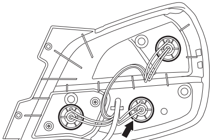
Rear turn-signal lamp socket
