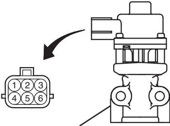
EGR valve
