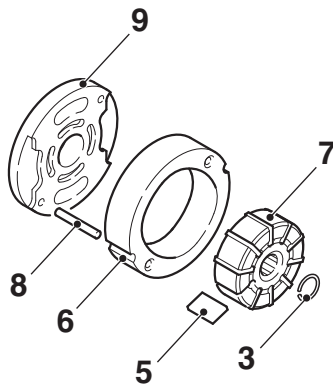
Oil pump cartridge kit
