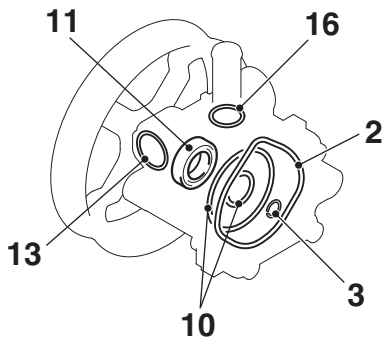
Oil pump seal kit
