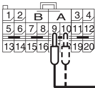
C-120 Harness side connector (rear view)
