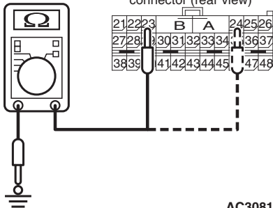
C-119 Harness side connector (rear view)
