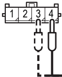
C-309 Harness side connector (rear view)
