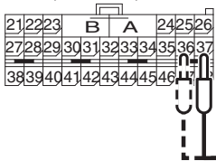
C-119 Harness side connector (rear view)
