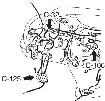
Harness side C-106
