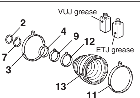
EBJ or VUJ boots repair kit
