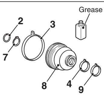
ETJ boots repair kit
