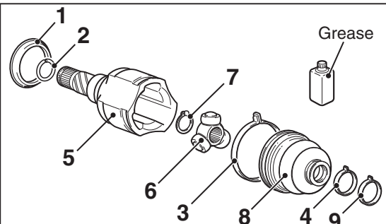
ETJ repair kit
