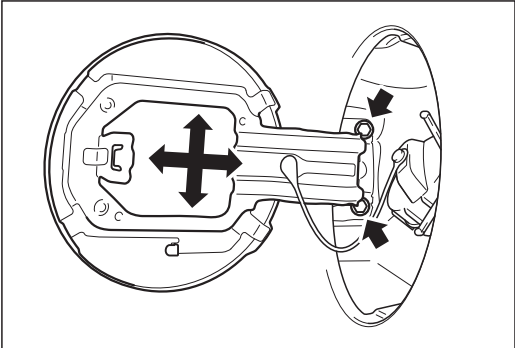
Fuel filler lid height and clearance adjustment
