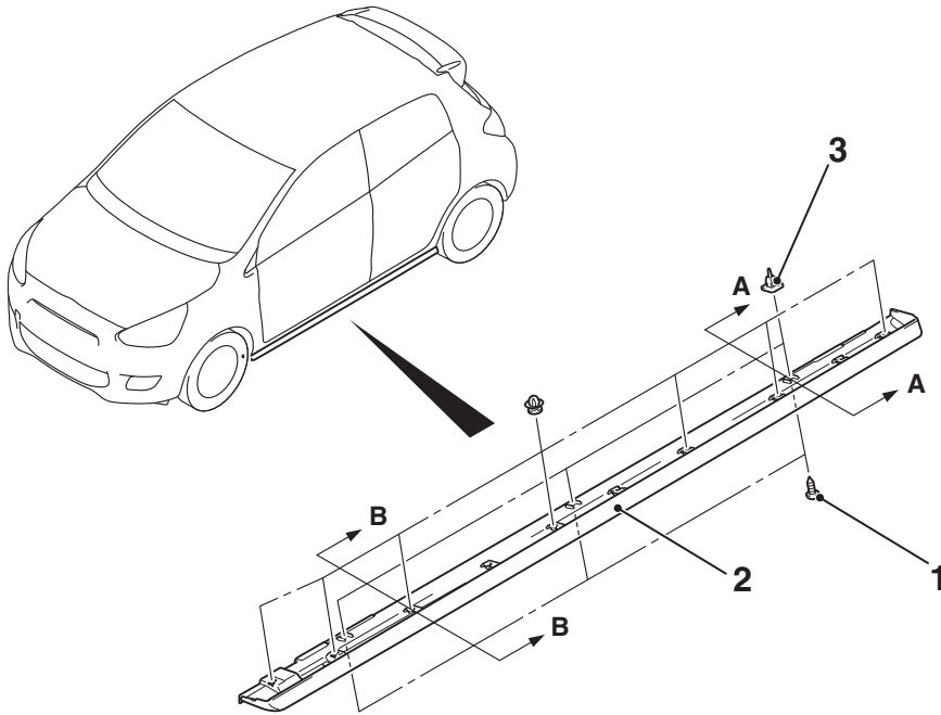
Double-sided tape affixed location
