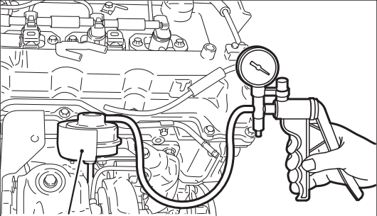
Variable geometry actuator
