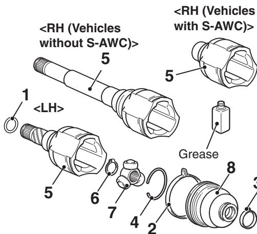
PTJ repair kit
