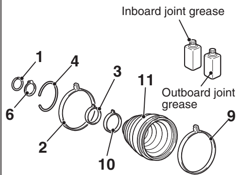
EBJ boots repair kit <LH, RH (Vehicles with S-AWC)>
