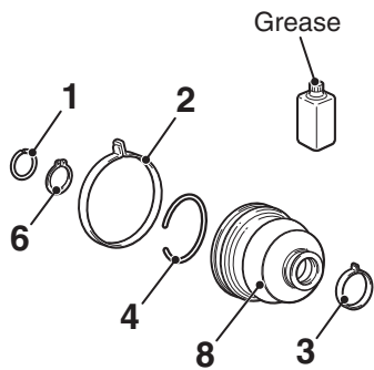
PTJ boots repair kit
