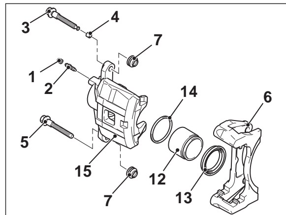
Brake caliper kit
