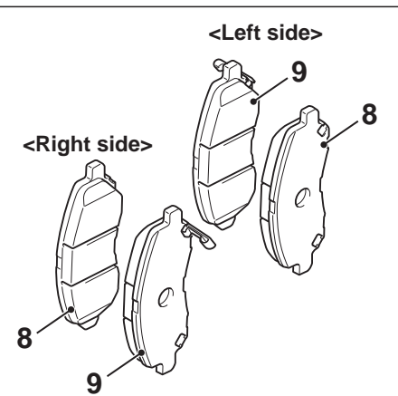
Pad set
