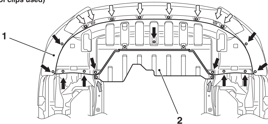
View A (Kinds of clips used)
