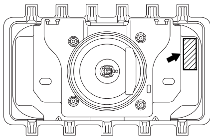
Passenger's (front) air bag module
