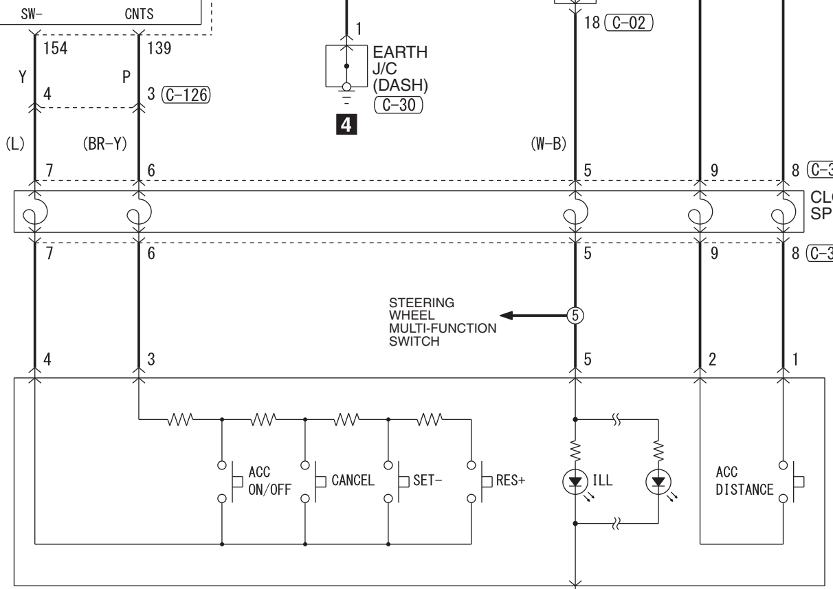
CRUISE CONTROL SWITCH (C-305)
