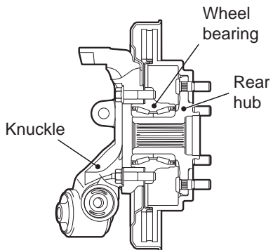
Vehicles with 16 inch brake
