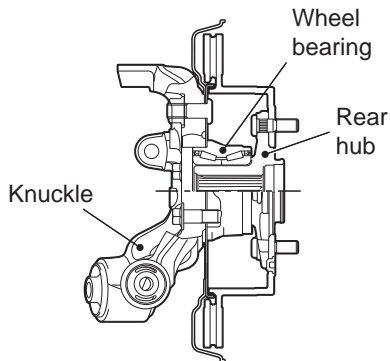
Vehicles with 17 inch brake
