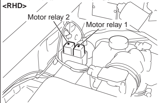
Motor relay 1
