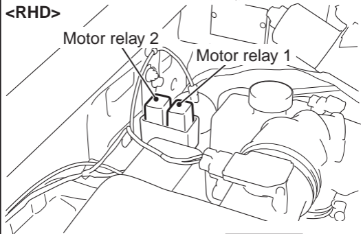
Motor relay 1, 2
