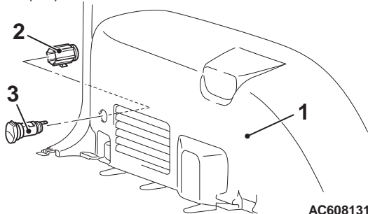
Lower quarter trim (LH) <Short wheelbase>
