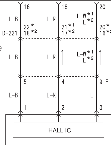
HEIGHT SENSOR (REAR) E-117
