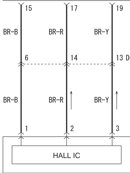
HEIGHT SENSOR (FRONT) A-22
