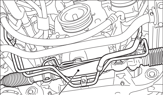
Power steering gear box assembly
