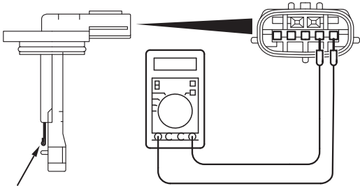
Intake air temperature sensor
