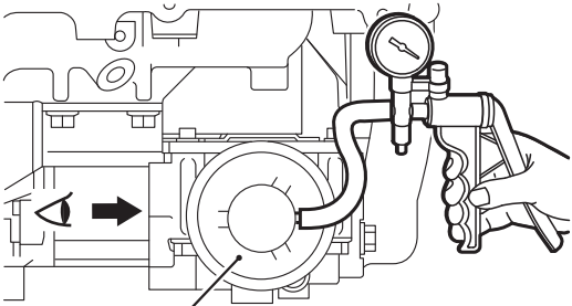
EGR valve vacuum actuator
