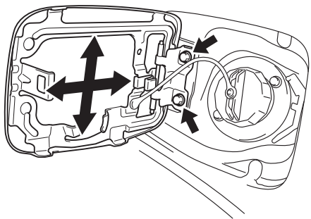
Fuel filler lid height and clearance adjustment
