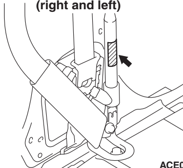
Lap pre-tensioner (right and left)
