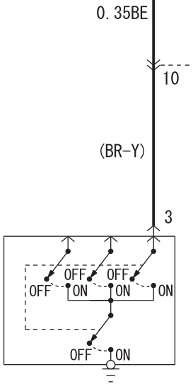
FRONT DOOR SWITCH (PASSENGER'S SIDE) (E-18)
