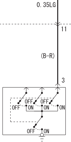
FRONT DOOR SWITCH (DRIVER'S SIDE) (E-04)
