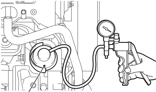
Variable geometry actuator
