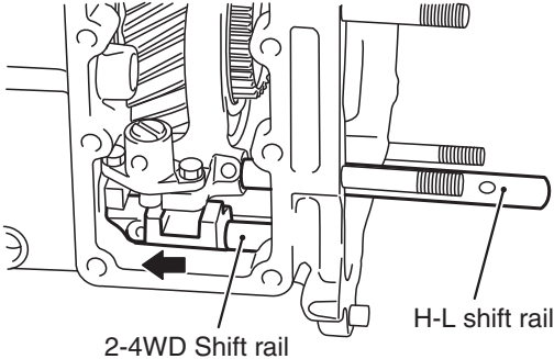
H-L shift rail
