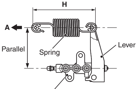
Load sensing proportioning valve
