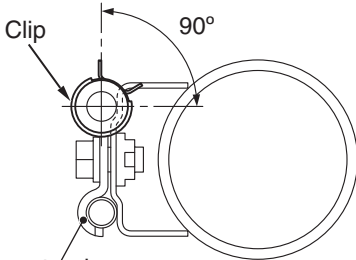
Power steering oil line bracket C
