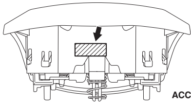
Driver's air bag module
